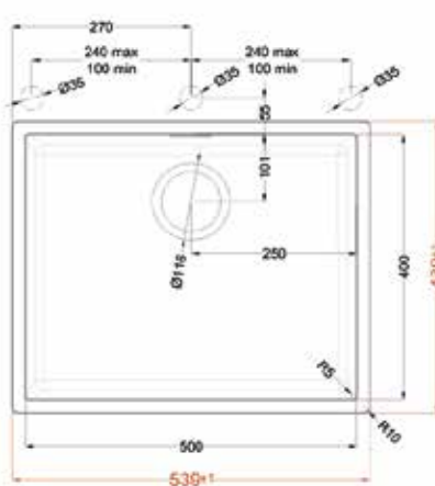
Pop-up Push Control Installation scheme for Medium type
